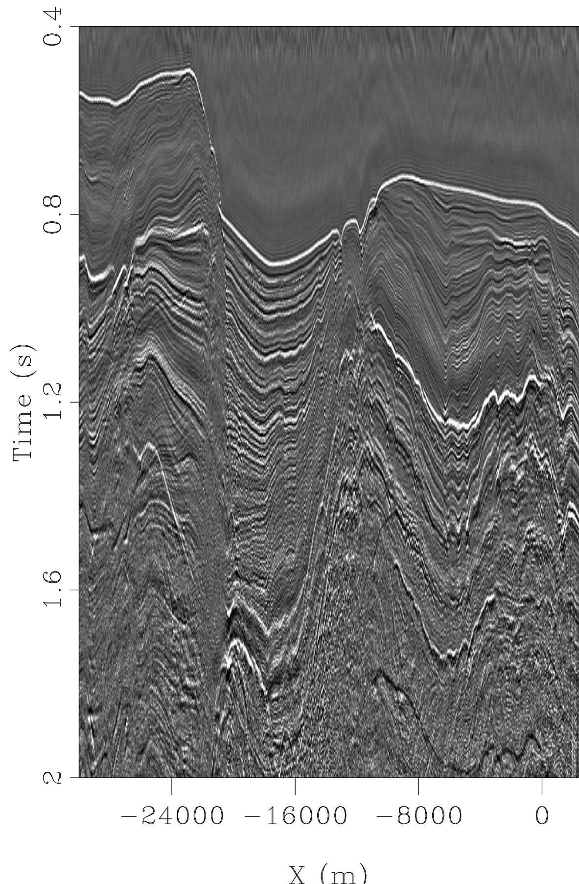
Deconvolved data
