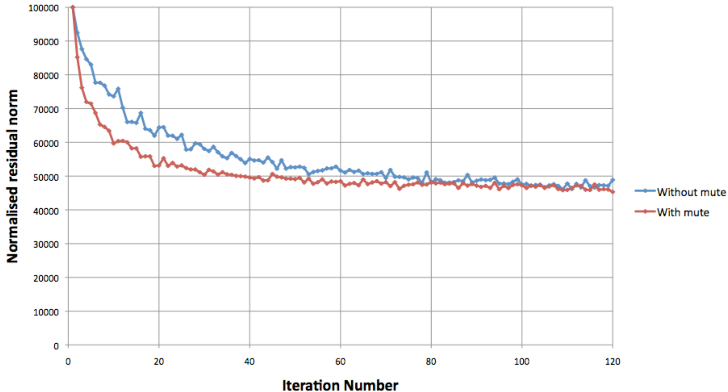
Phase encoded data space residuals with iteration number
