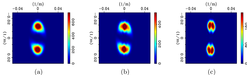
Figure 13: Wavenumber domain point-spread-functions at point x = 2600 m and z = 2600 m for the (a) baseline and (b) monitor. Note in the difference PSF (c), that there is significant illumination differences at various wavenumbers. [CR]
