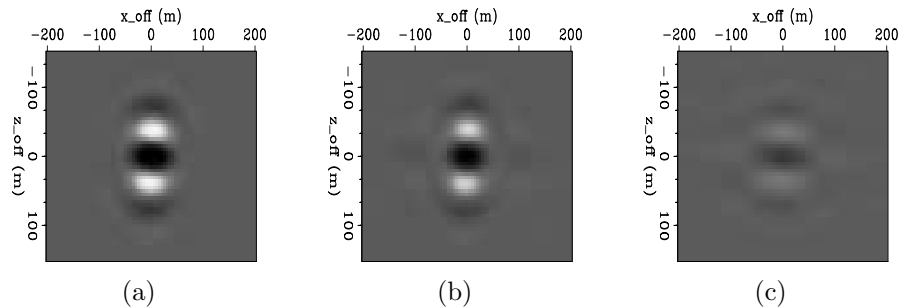
Figure 12: Point-spread-functions at point x = 2600 m and z = 2600 m for the (a) baseline and (b) monitor. Note in the difference PSF (c), that there is significant energy away from the center of the PSF (i.e. in the off-diagonal parts of the Hessian). [CR]
